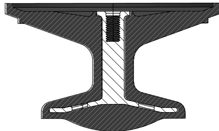
SECTION VIEW
